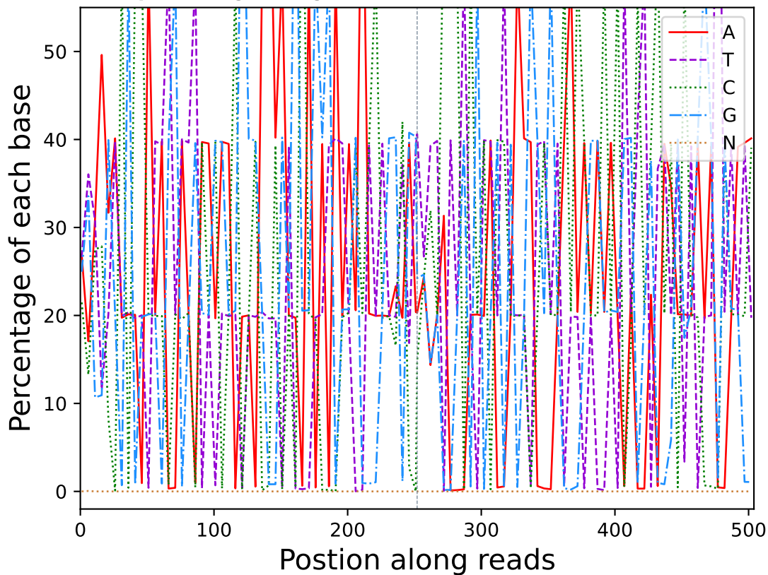
Base percentage along reads (R10813)
